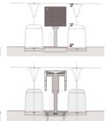
SECTION
